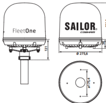
SAILOR Fleet One Above Deck Unit (3,9 kg)
